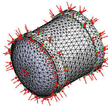
After Meshing
